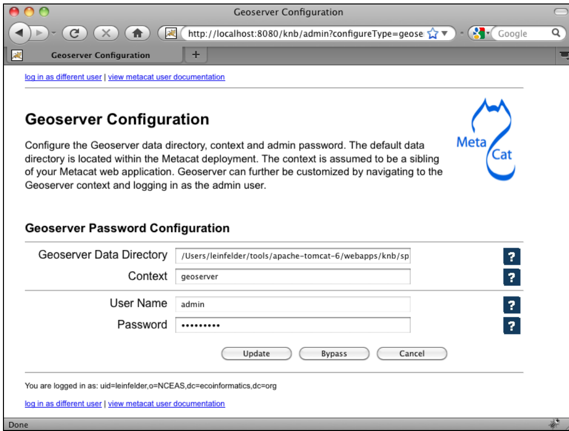
Figure 3.11: Configuring Geoserver.
